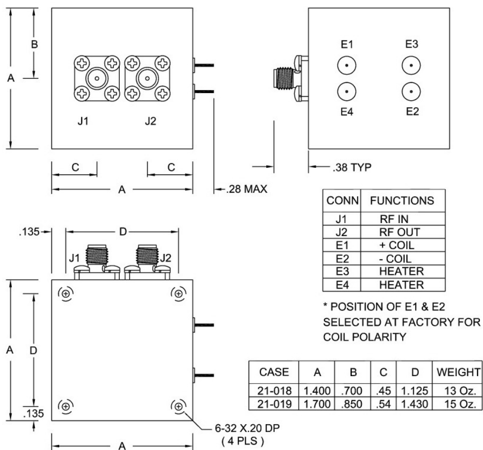
CASE DRAWING 21-018 / 21-019
