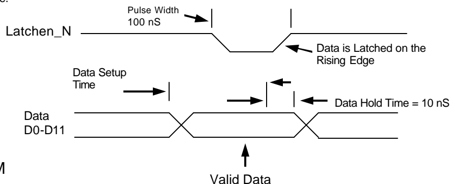
TIMING DIAGRAM
